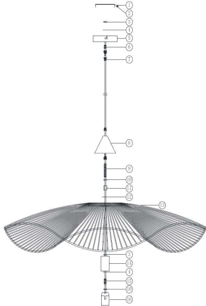
FR / 1. Encastrez la tige filetée ENG / 1. Embed the threaded rod
