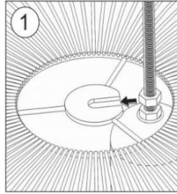
FR / 1. Encastrez la tige filetée ENG / 1. Embed the threaded rod
