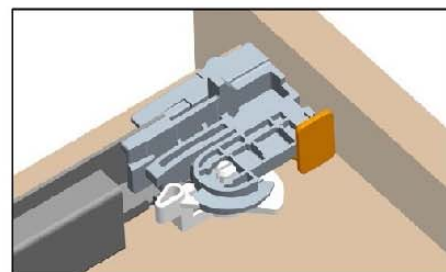
Réglage vertical + 3mm / Vertical adjustment + 3mm / Verticale aanpassing + 3mm
