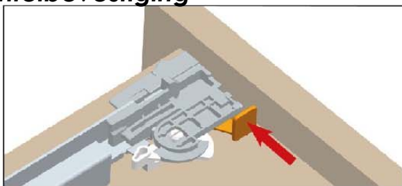
Fixation anti basculement / Anti-tilt mounting / Anti-kantelbevestiging
