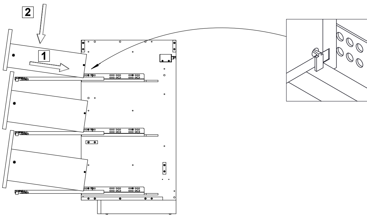
Fixation anti basculement / Anti-tilt mounting / Anti-kantelbevestiging
