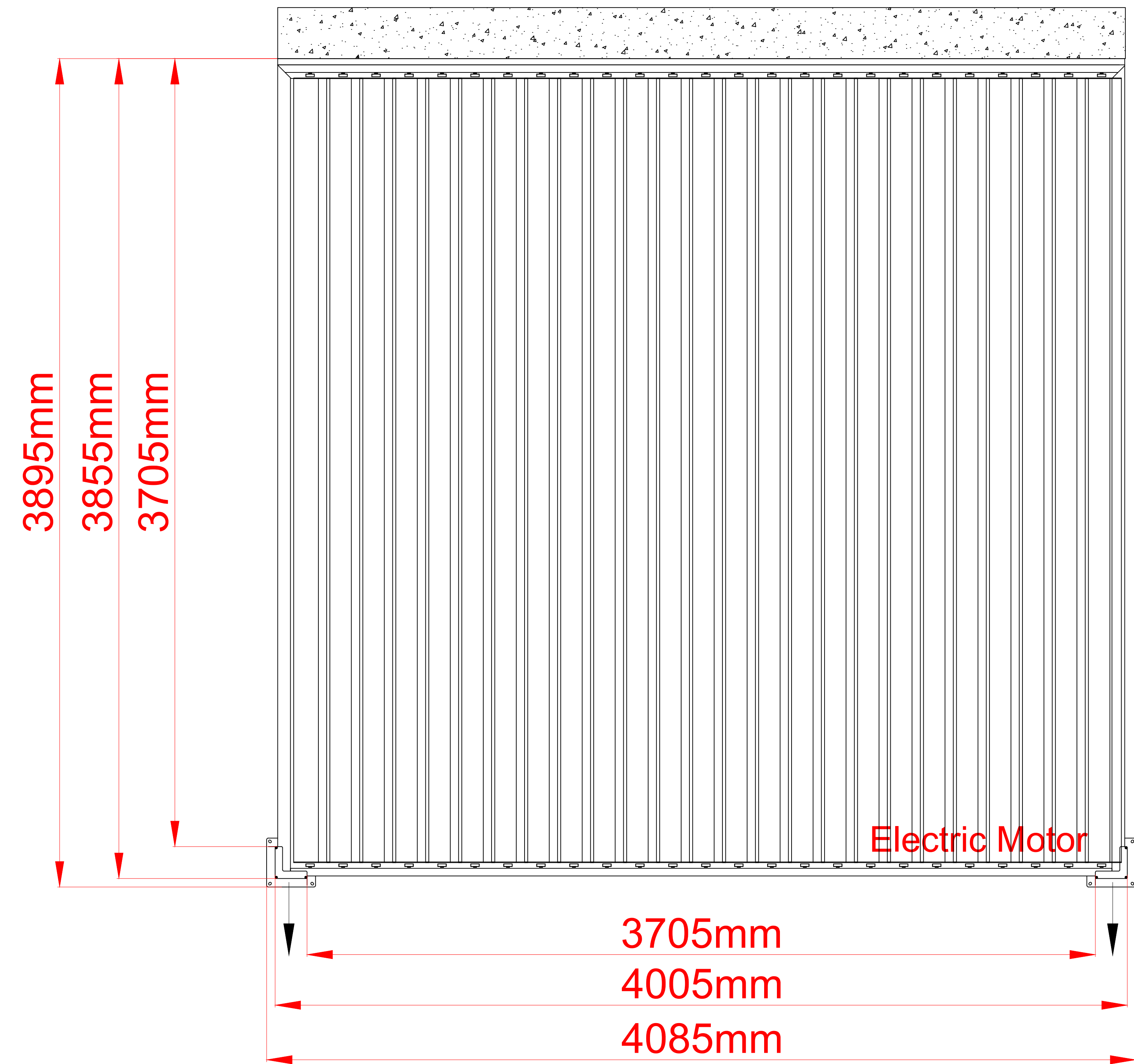
PLAN VIEW
