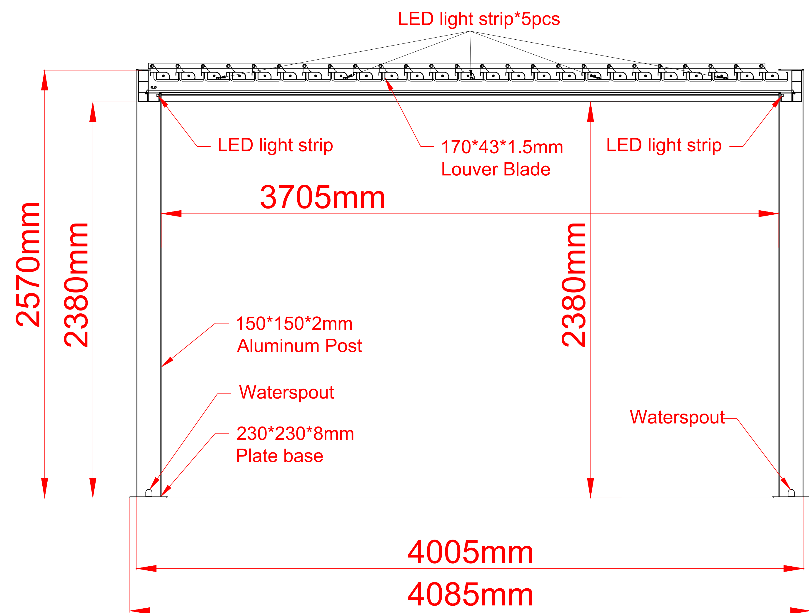
ELEVATION VIEW
