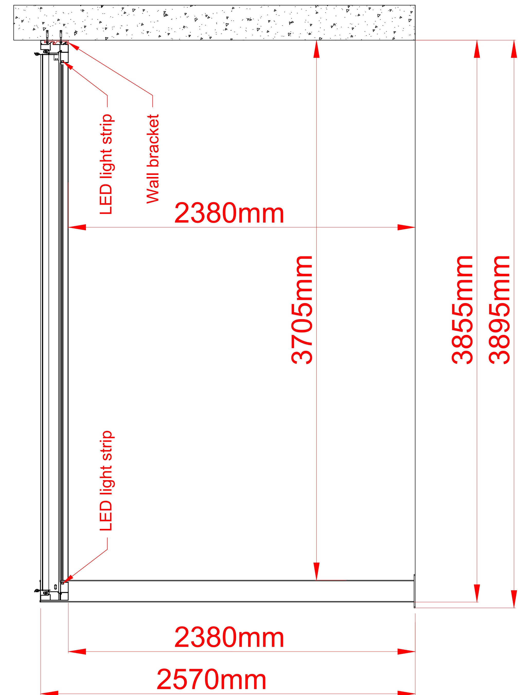
ELEVATION VIEW
