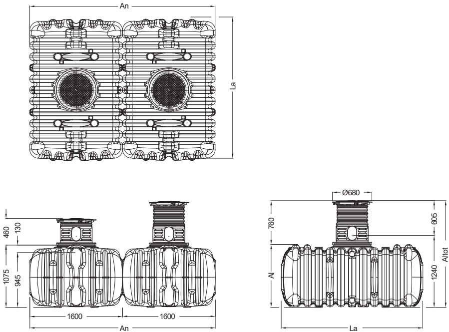
Fig.5: Dimensiones – FLAT M
