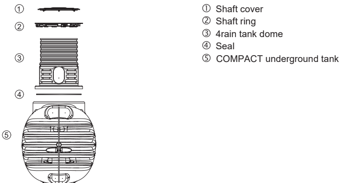
Fig. 16: Components – COMPACT
