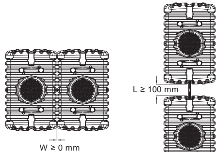
Fig. 23: Interconnecting multiple tanks – FLAT
