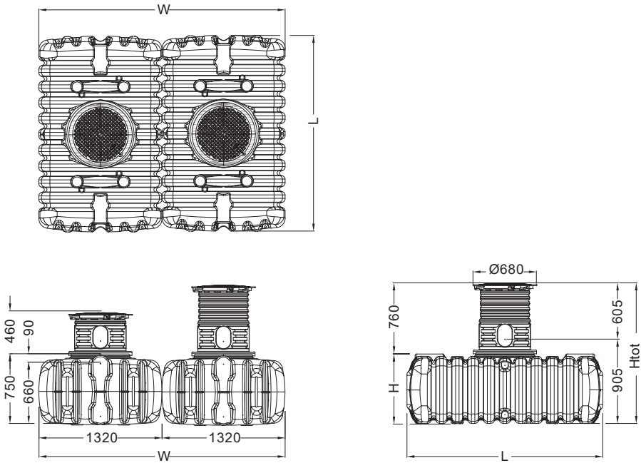
Fig. 4: Measurements – FLAT S
