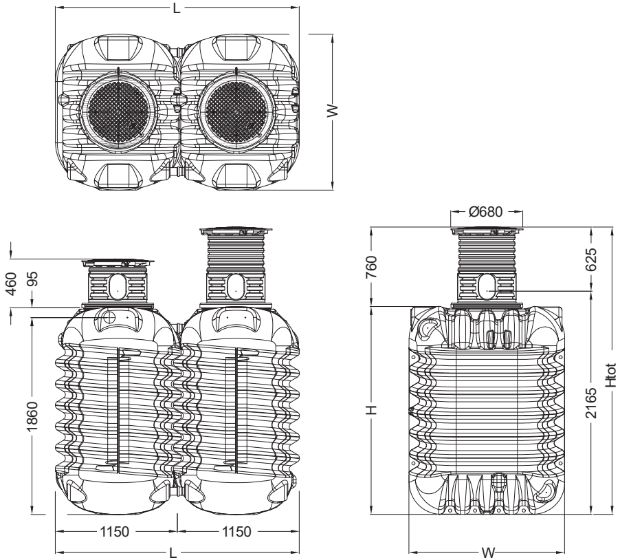
Fig. 7: Measurements – MODULARIS
