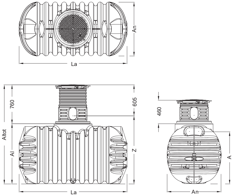
Fig.8: Dimensiones – COMPACT
