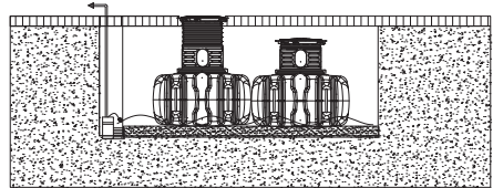
Fig. 20: Installation in a pit carrying water – example with FLAT
