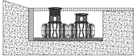
Fig. 19: Installation on a slope – example with FLAT
