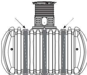
Fig. 13: Section through support pipes – FLAT L
