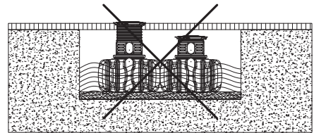
Fig. 3: Ground/stratum water – example with FLAT
