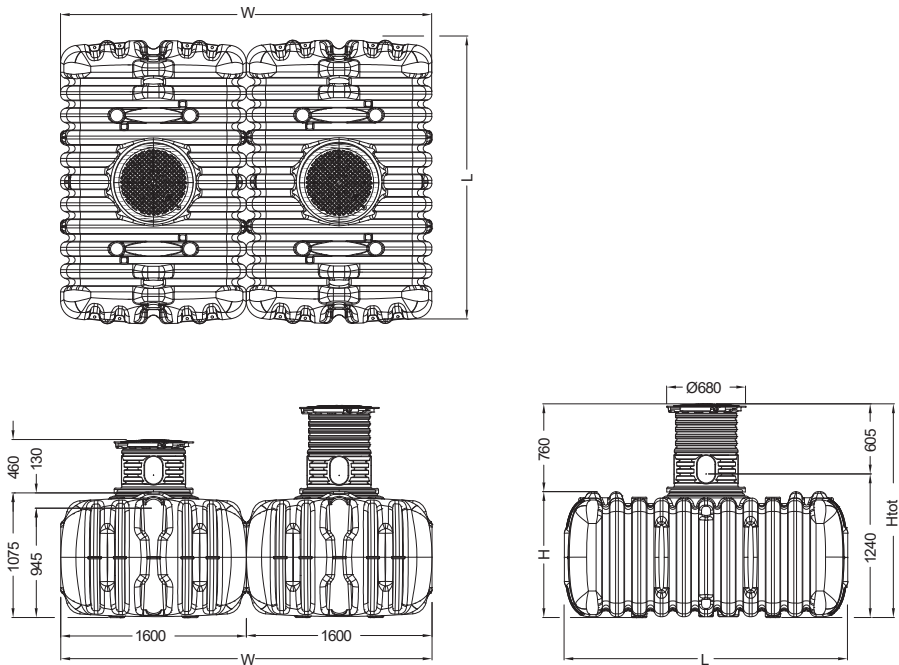
Fig. 5: Measurements – FLAT M
