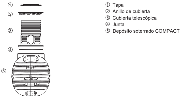
Fig. 16: Componentes – COMPACT
