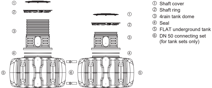
Fig. 10: Components – FLAT
