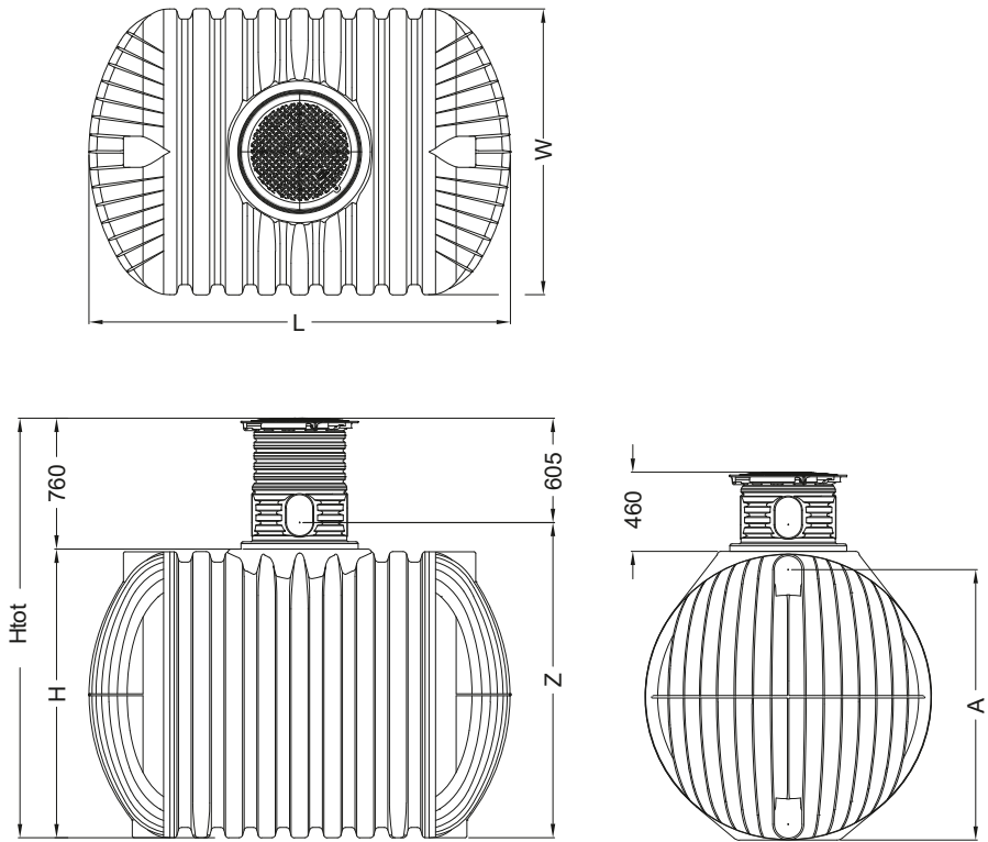
Fig. 9: Measurements – PROFI
