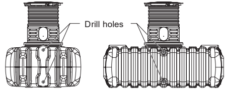
Fig. 22: Drill holes for interconnecting multiple tanks – FLAT
