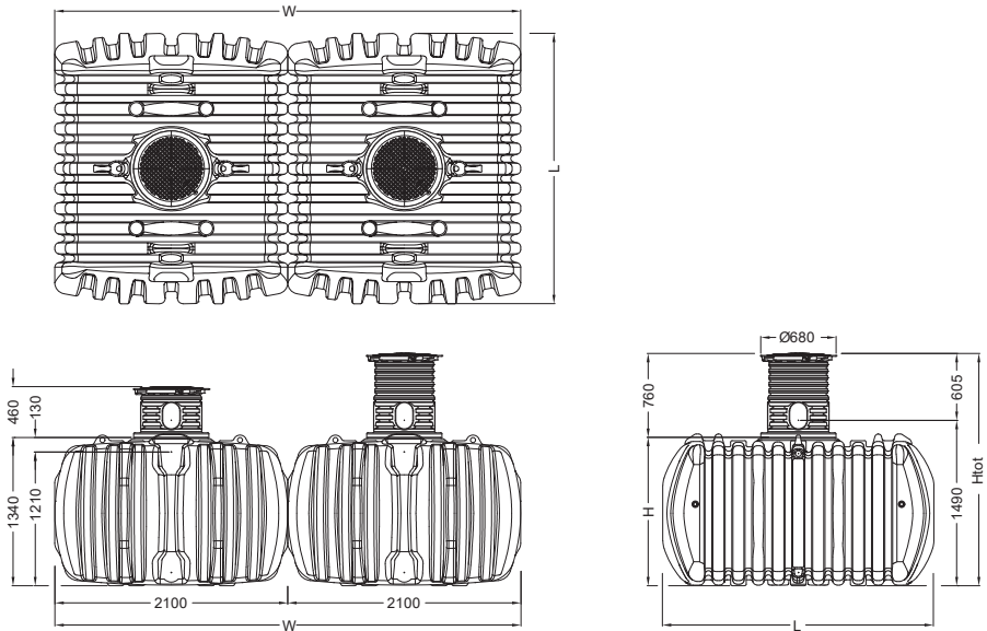
Fig. 6: Measurements – FLAT L
