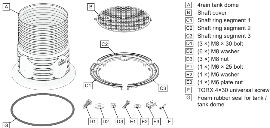
Fig. 32 – Tank dome and cover – parts overview
