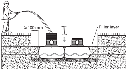
Fig. 27: Insertion and filling – FLAT
