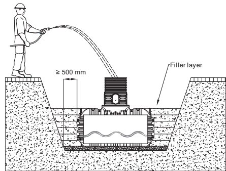
Fig. 30: Insertion and filling – COMPACT, PROFI
