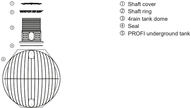
Fig. 17: Components – PROFI
