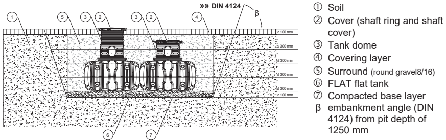
Fig. 18: Recommended installation – example with FLAT
