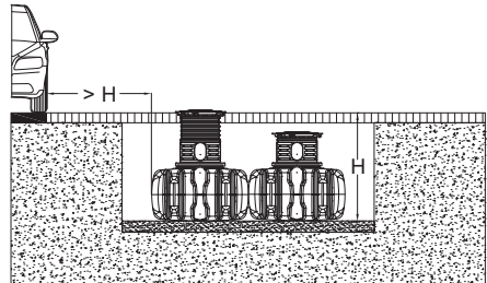
Fig. 21: Distance from roadways – example with FLAT
