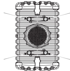
Fig. 12: Support pipe positions – FLAT S/M
