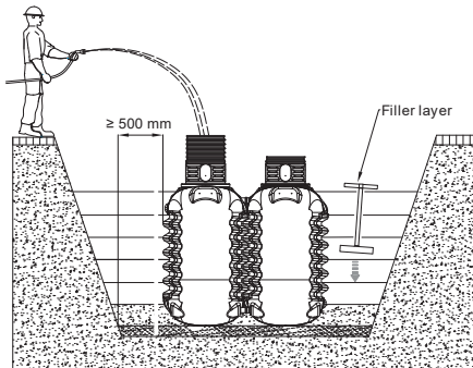
Fig. 29: Insertion and filling – MODULARIS
