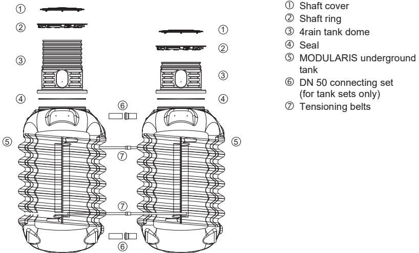
Fig. 15: Components – MODULARIS
