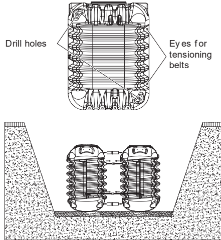
Fig. 24: Interconnecting multiple tanks – MODULARIS
