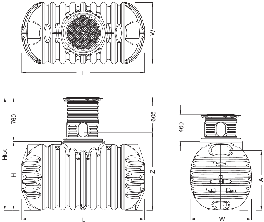
Fig. 8: Measurements – COMPACT
