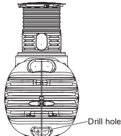
Fig. 25: Interconnecting multiple tanks – COMPACT
