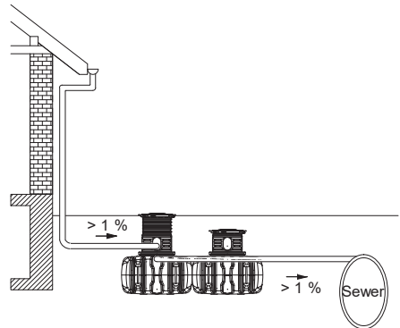
Fig. 31 – Recommended connections – example with FLAT
