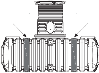
Fig. 11: Section through support pipes – FLAT S/M
