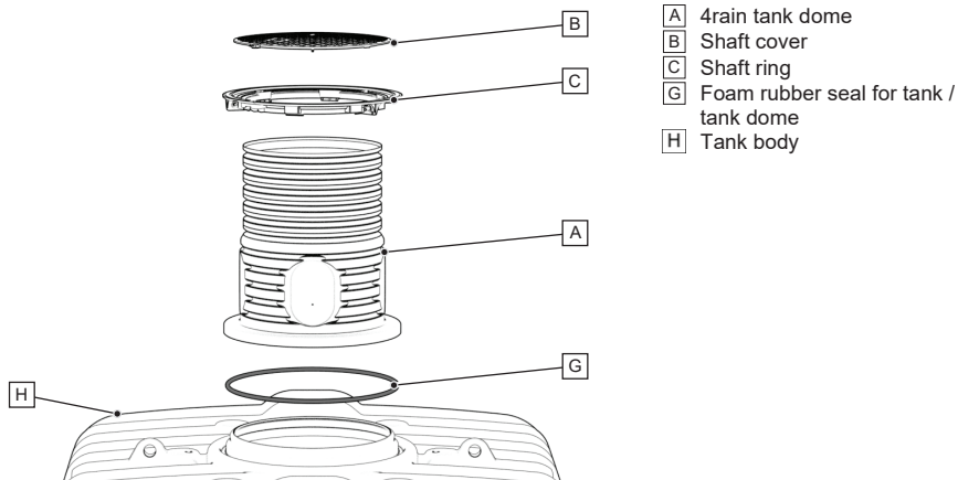
Fig. 33 – Tank dome and cover – assembly overview
