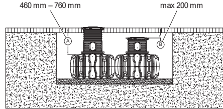
Fig. 1: Covering heights – example with FLAT
