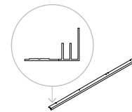
[C2]x4 1557mm
