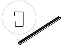
[K9]x2 1653mm
