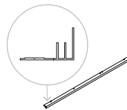
[C1]x4 2157mm
