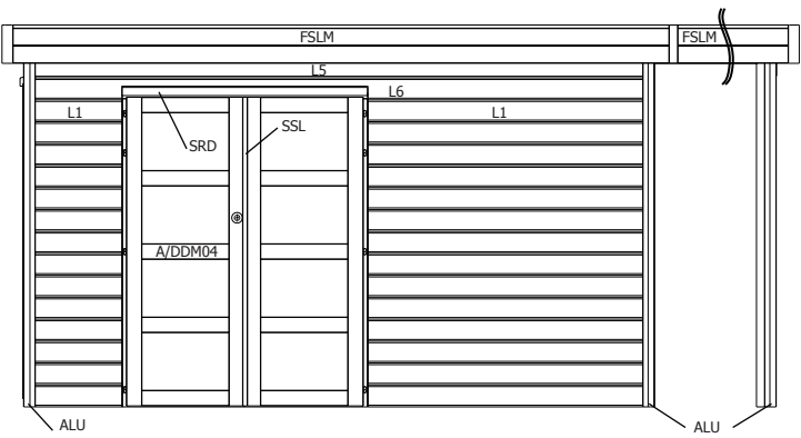
FACADE
