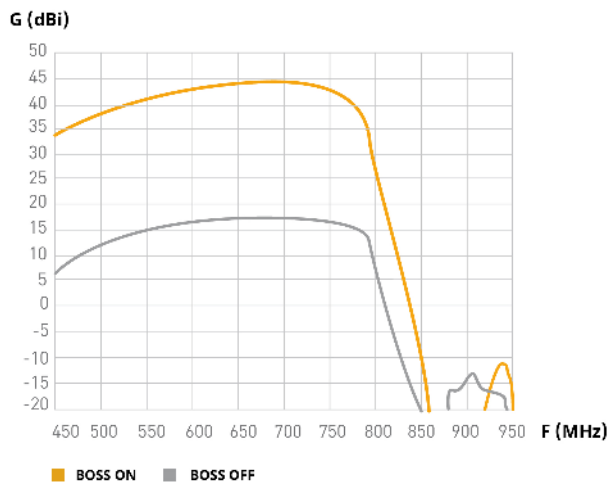
Radiation pattern
