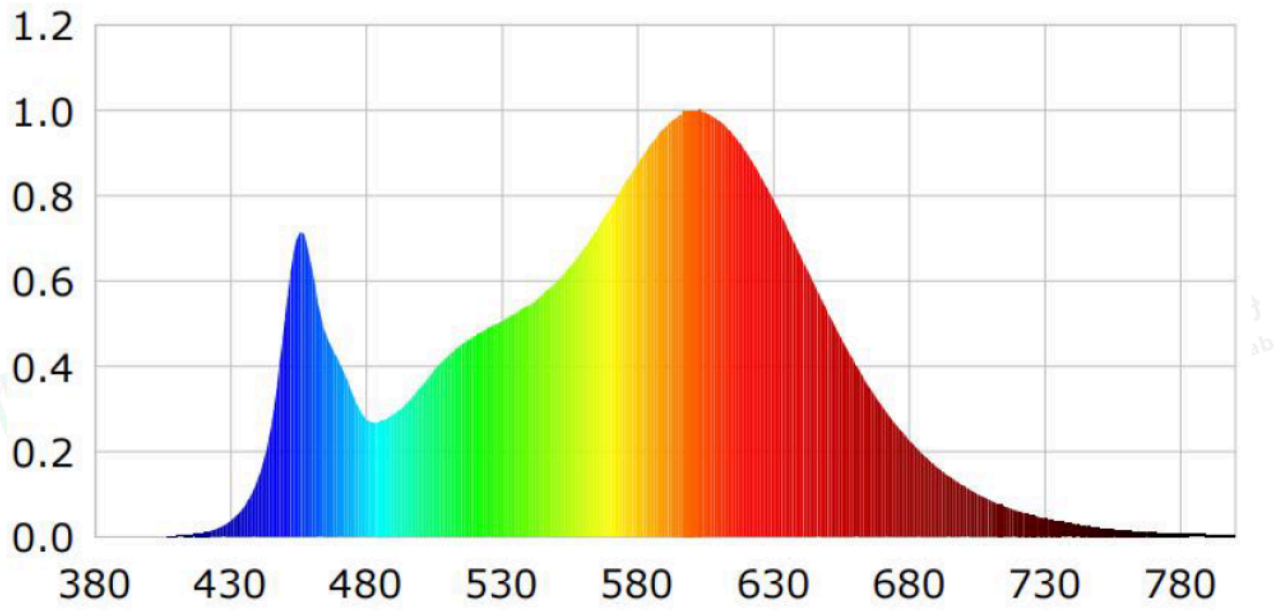
Spectral power distribution(3000K)
